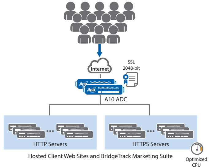
SapientNitro Optimized Network Overview
