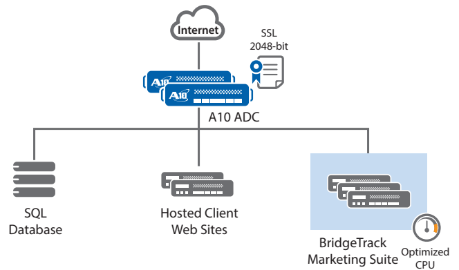
SapientNitro Optimized Network Overview
